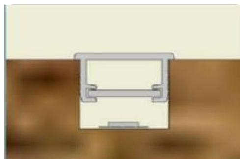
BAN 14515 used as a light diffuser with LED strip placed underneath
