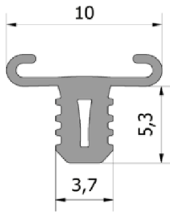
ABS U 1062 T LED carrier profile with 8 mm wide LED strip.
