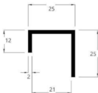
ABS U 252512
